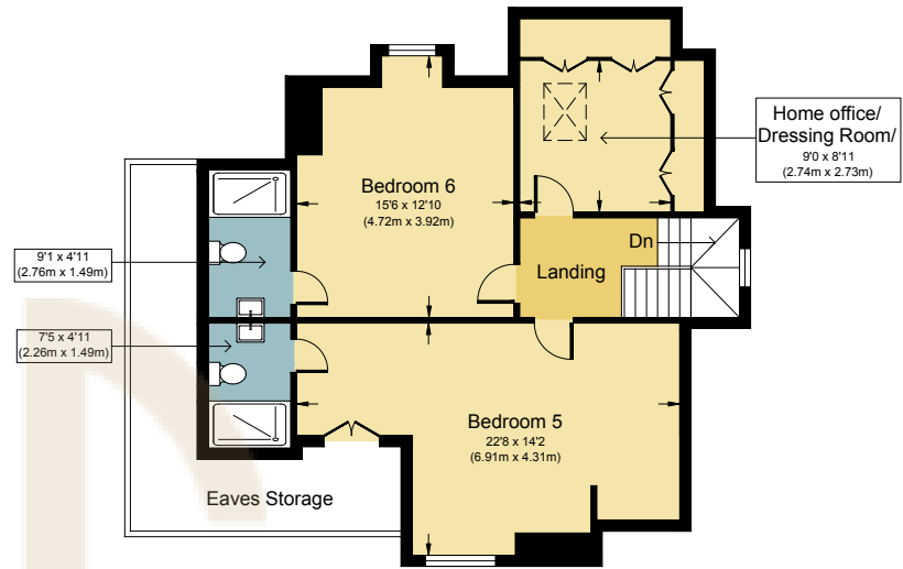
Second Floor
