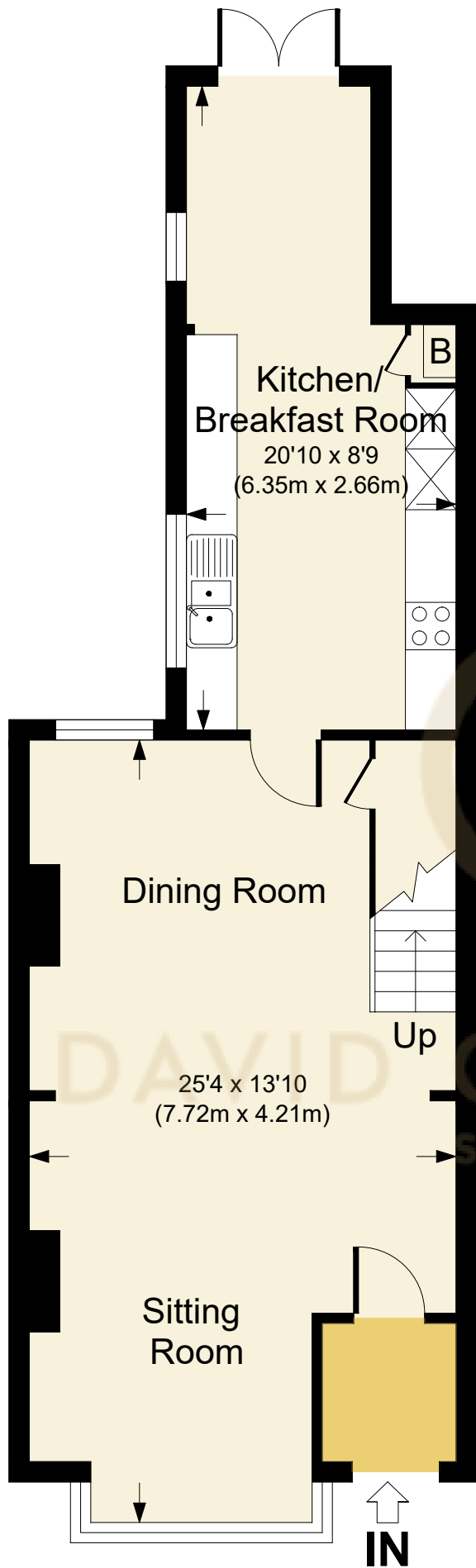
Ground Floor
